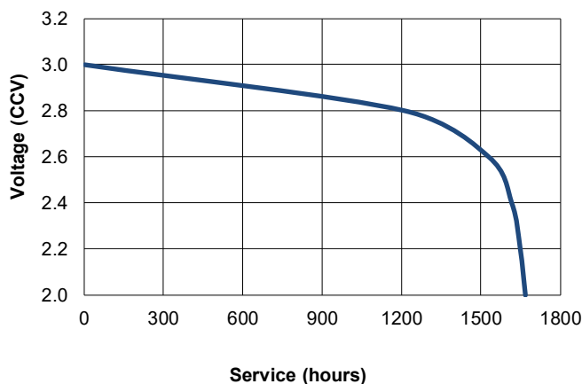
RATING DRAIN 7.5K Ohms continuous to 2V
