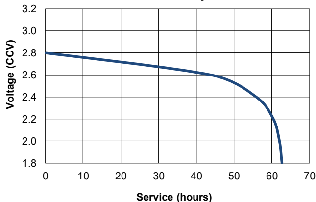
KEY FOB 10mA 5s/min 24h/day to 1.8V
