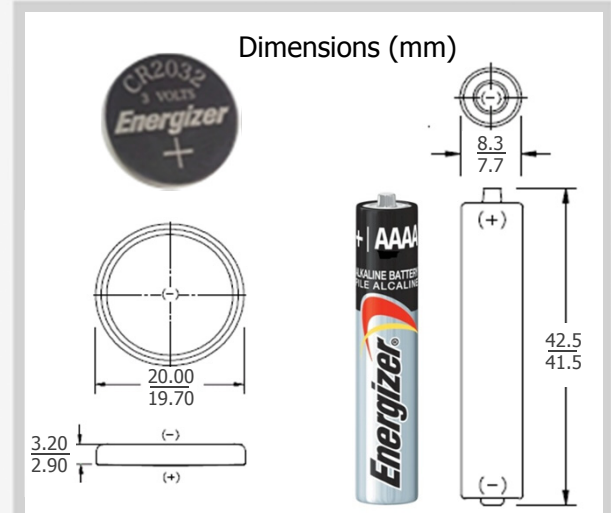
CR2032 / AAAA Alkaline
