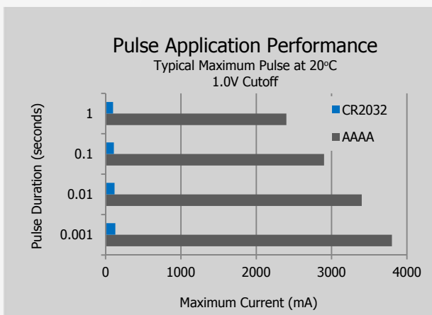
Pulse Capability
