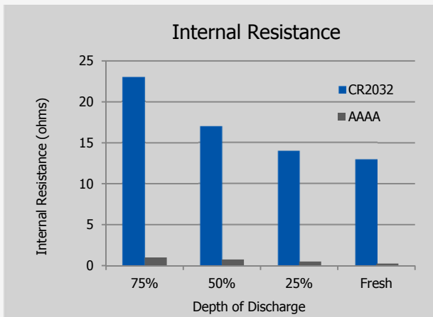
Internal Resistance
