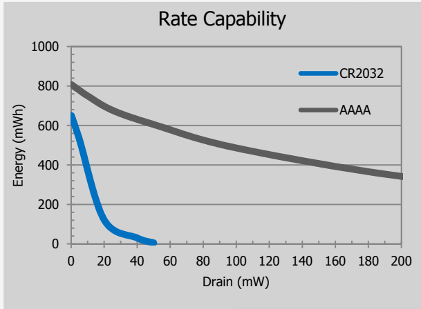
Rate Capability
