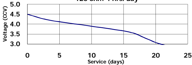
TYPICAL DISCHARGE 125 ohm 4 hrs/day
